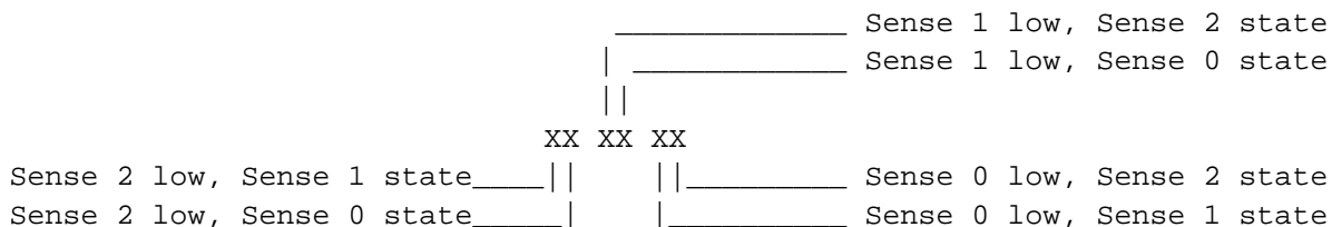
Figure 1-Extended Type-7 Sense Line Decode Method
