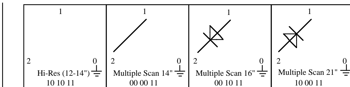
Figure 4—Extended Type 6 Sense Line Decode Diagram
