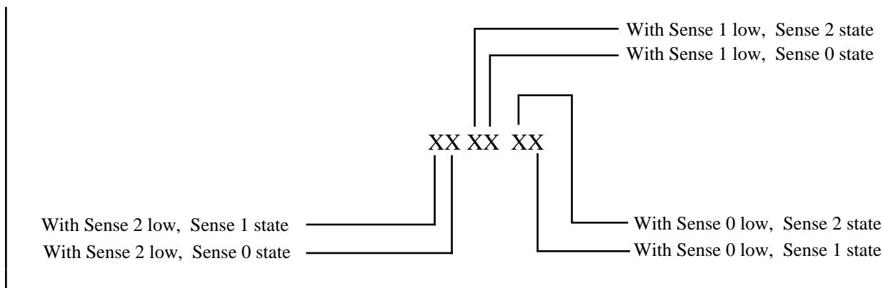
Figure 1—Extended Type-7 Sense Line Decode Method
