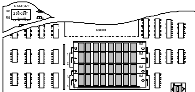
Figure 1 - Macintosh Plus Memory Configurations
