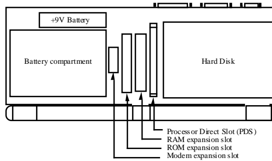
Figure 6 - Macintosh IIcx, IIci, and Portable Memory Configurations
