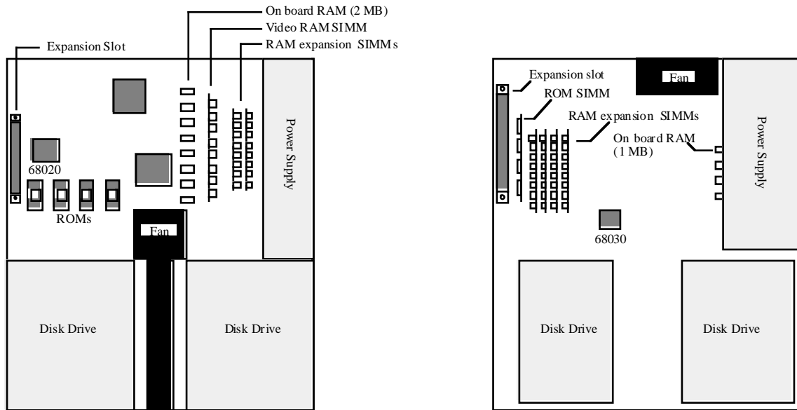
Macintosh LC (RAM SIMMs must be 100 nS RAS-access time or faster.)
