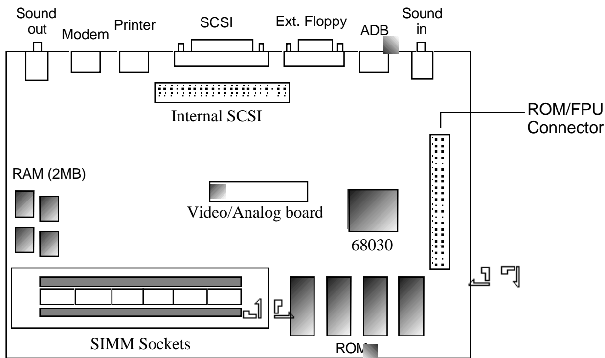
Figure 10 - Macintosh Classic II (SIMMs must be 100 ns RAS-access time or faster.)
