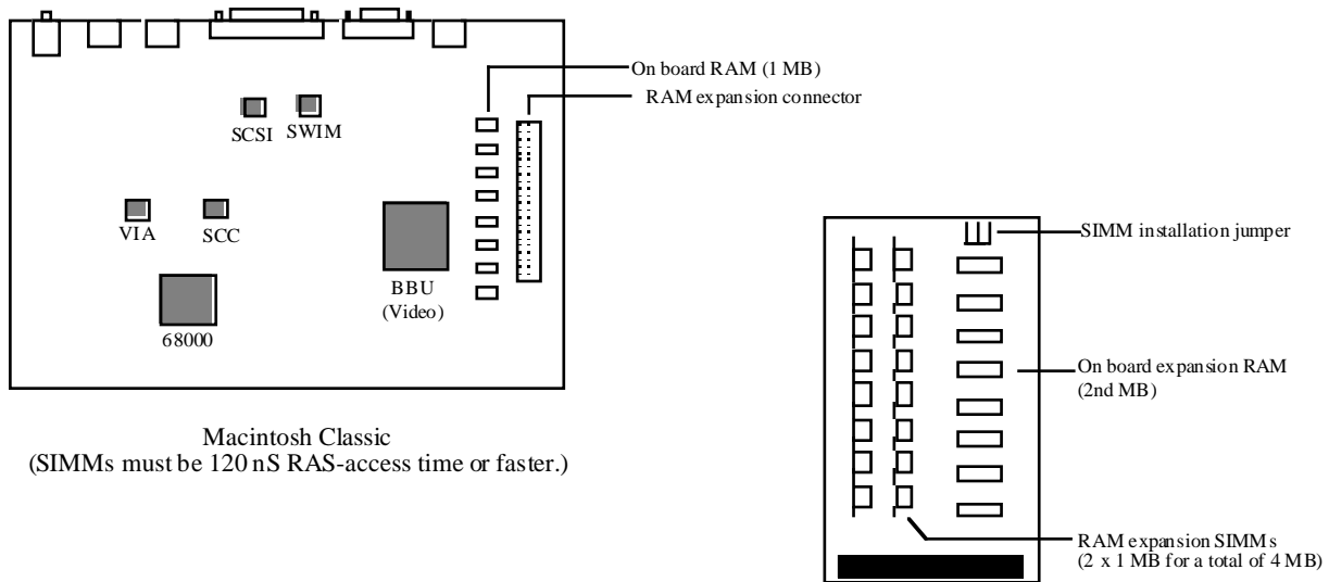
Macintosh Classic RAM expansion board
