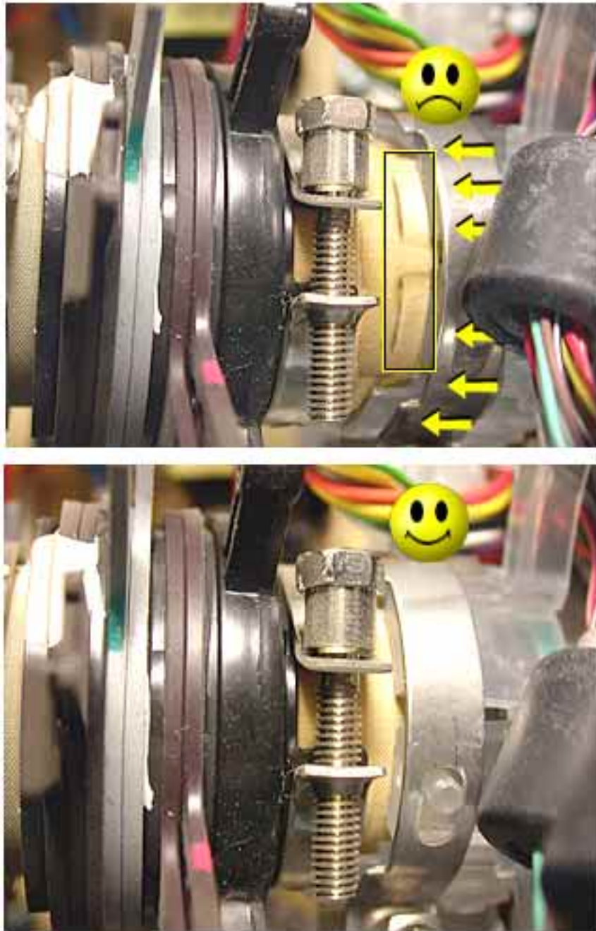
Figure 2 Video Board Improperly and Properly Seated
