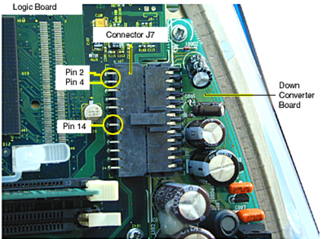
Testing Voltages at J7 on the Logic Board
