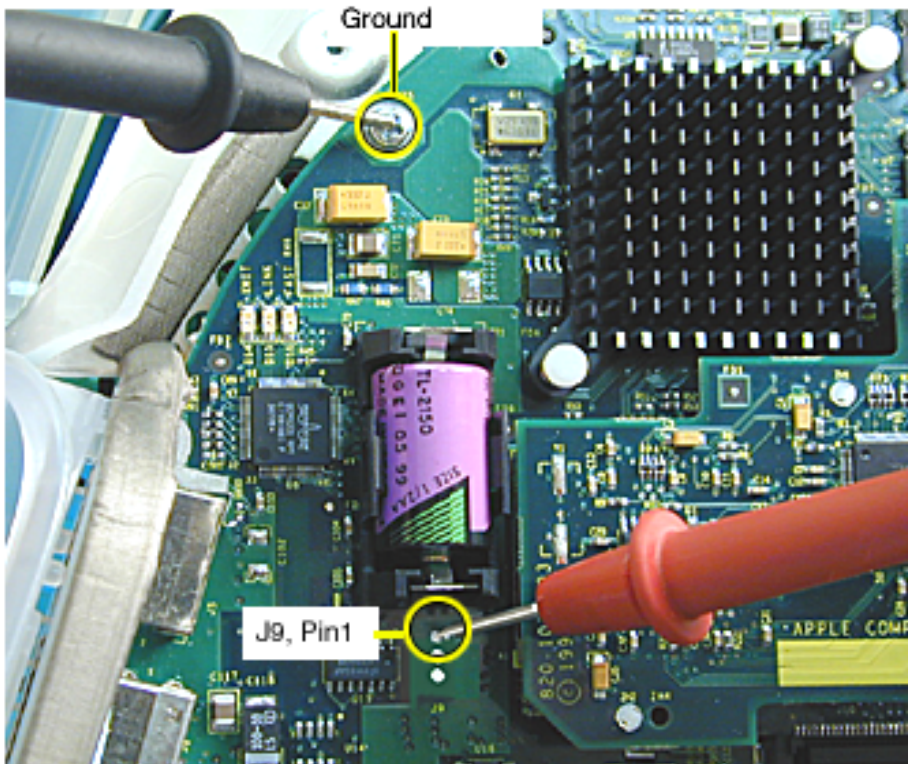
Testing for +5 V Trickle Power at J9 on the Logic Board
