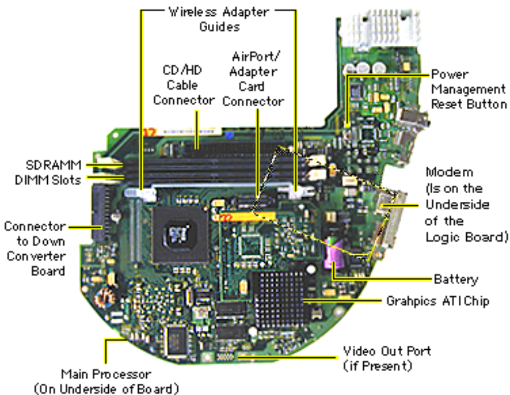
iMac Logic Board Diagram
