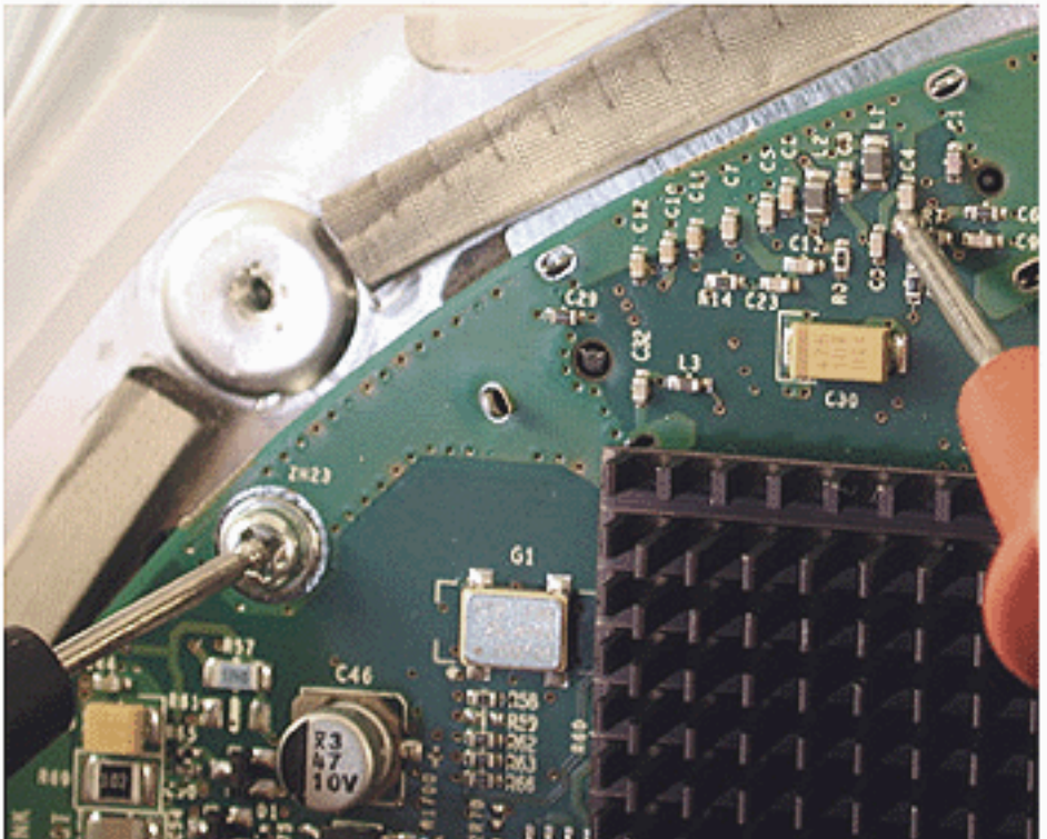
Testing DCO Voltages at C4 on the Logic Board
