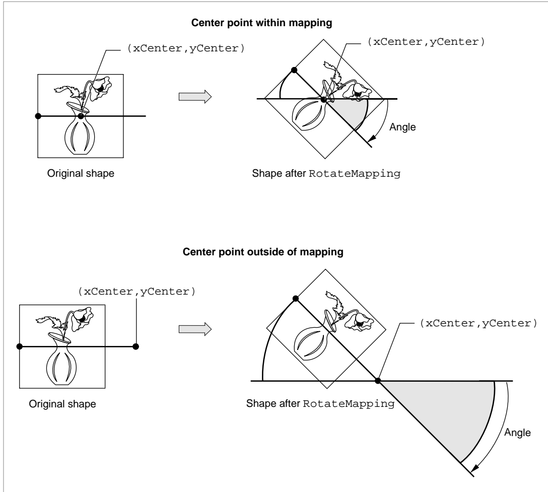
Figure 8-14 Rotating about different center points
