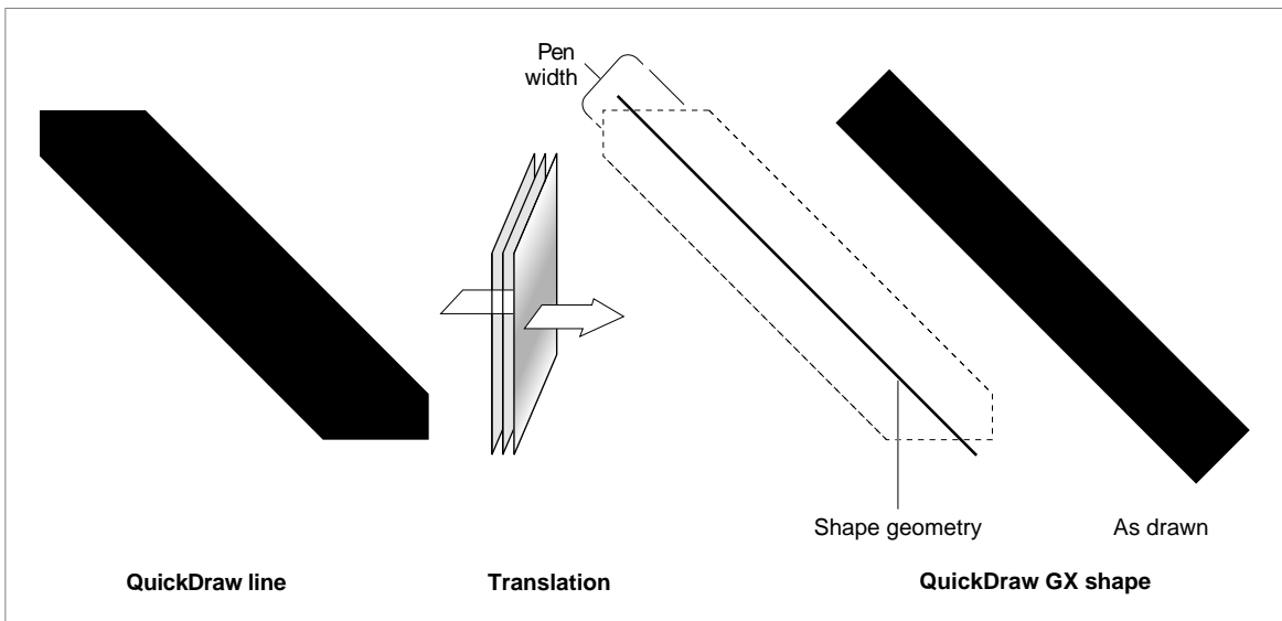
Figure 1-5 Translation of the QuickDraw line using gxReplaceLineWidthTranslation
