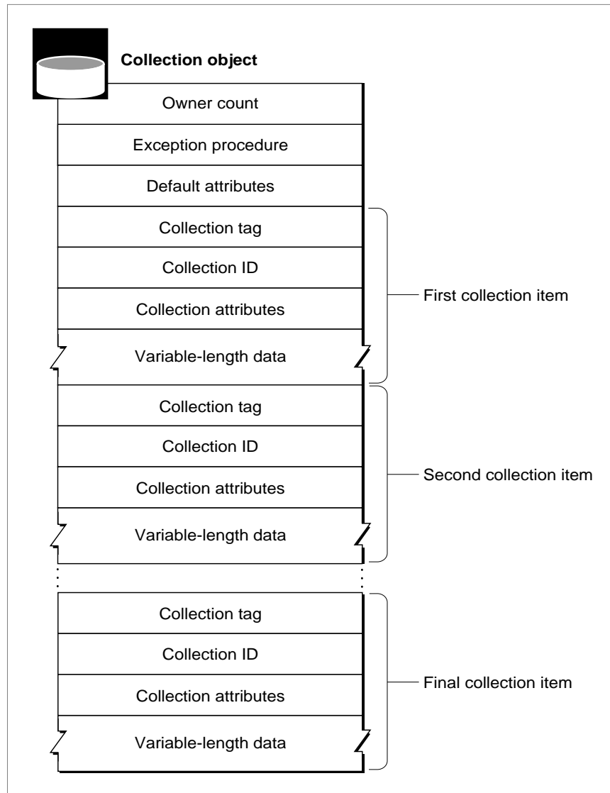
Figure 5-1 The collection object
