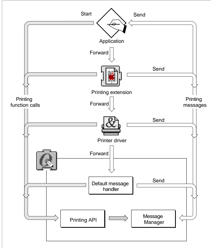
Figure 6-2 Printing with QuickDraw GX
