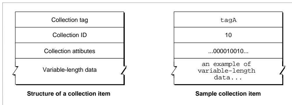
Figure 5-2 The collection item
