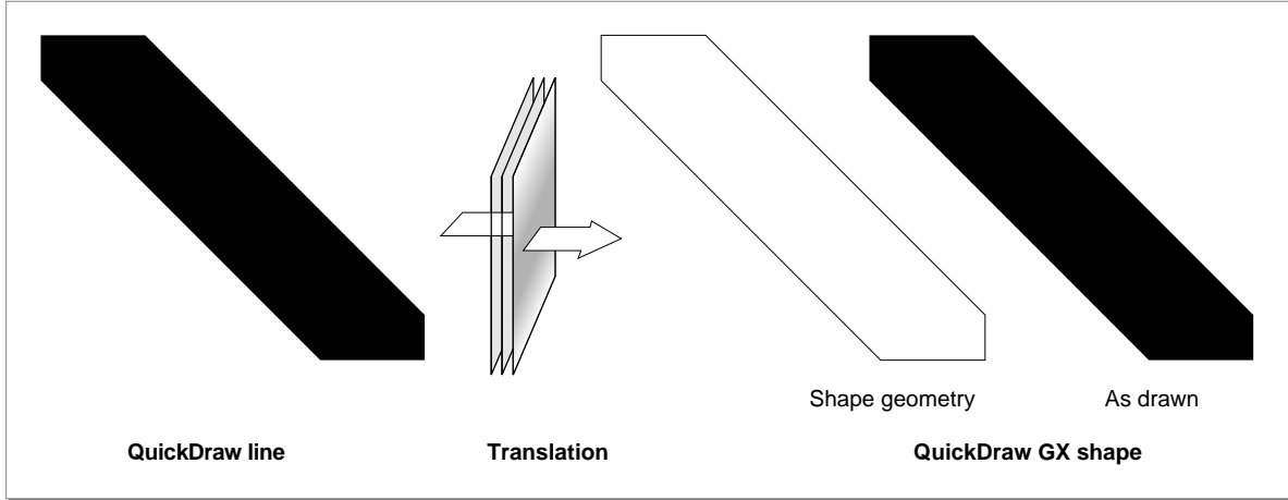
Figure 1-3 Translation of the QuickDraw line using gxDefaultOptionsTranslation
