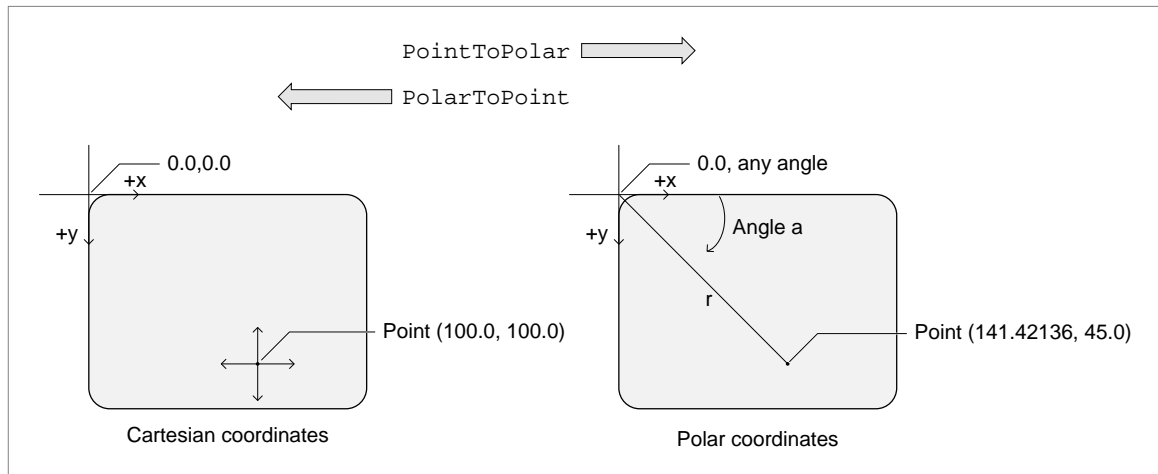
Figure 8-19 Converting between Cartesian and polar coordinates
