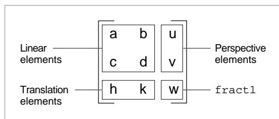
Figure 8-3 Mapping matrix elements
