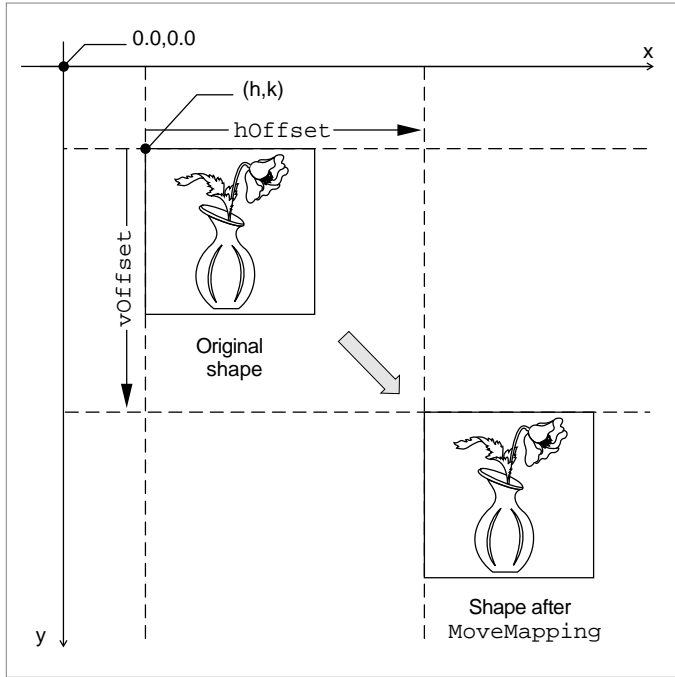
Figure 8-8 Translation by a relative amount with MoveMapping
