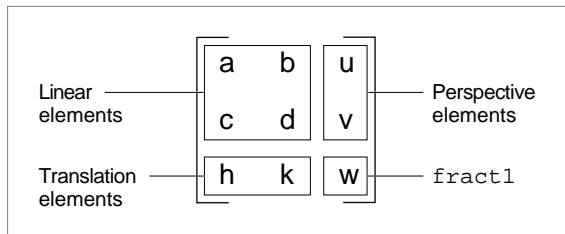
Figure 7-10 Mapping matrix elements
