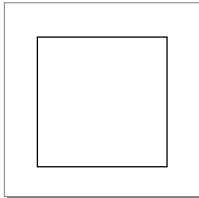
Figure 7-14 The rectangle shape drawn
