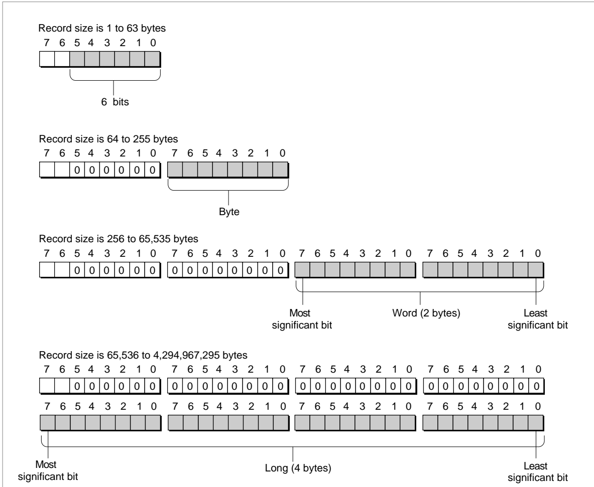
Figure 7-4 Data format of the record size
