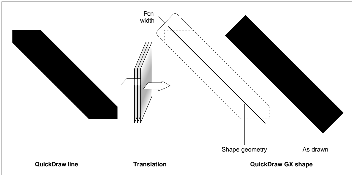
Figure 1-4 Translation of the QuickDraw line using gxSimpleGeometryTranslation
