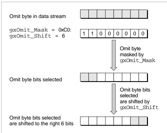
Figure 7-8 Select the bits from the omit byte
