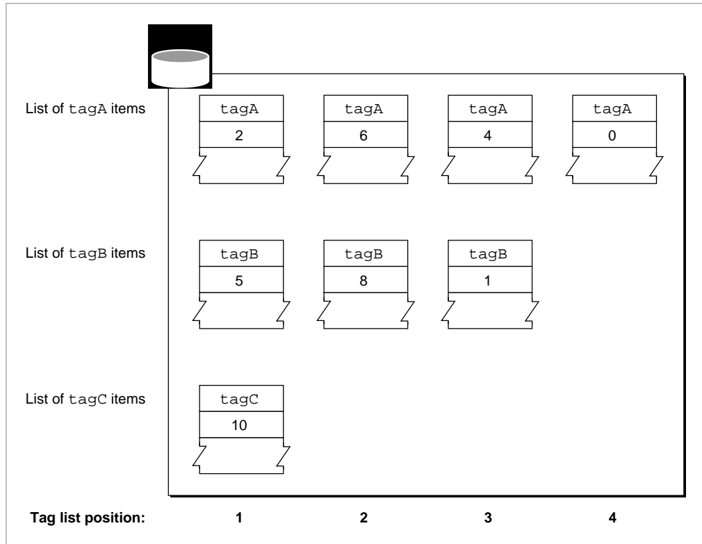
Figure 5-4 Items in a collection
