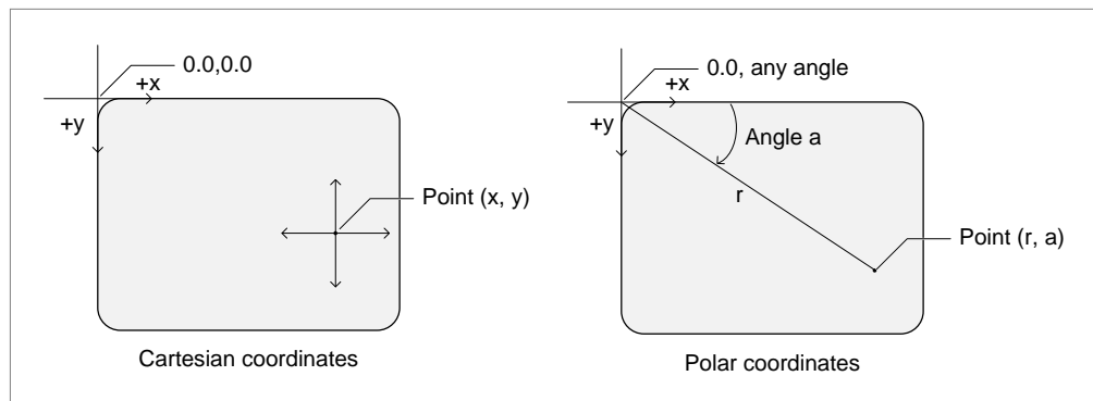
Figure 8-1 Cartesian and polar coordinates
