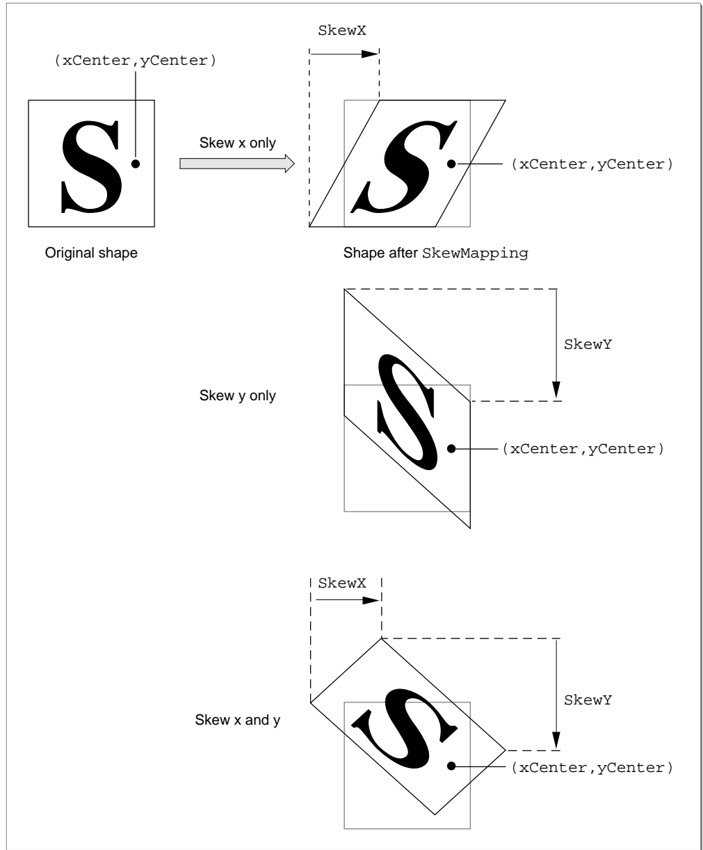
Figure 8-16 Skewing a shape both horizontally and vertically
