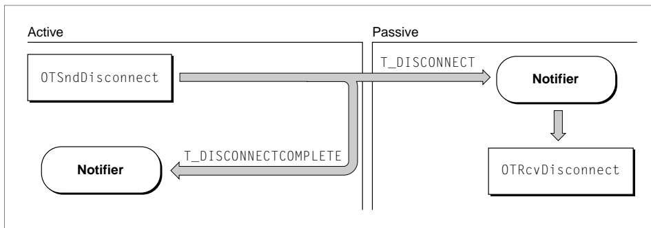
Figure 4-5 An abortive disconnect
