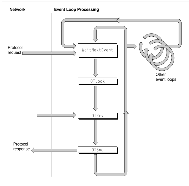
Figure 5-2 Polling for events
