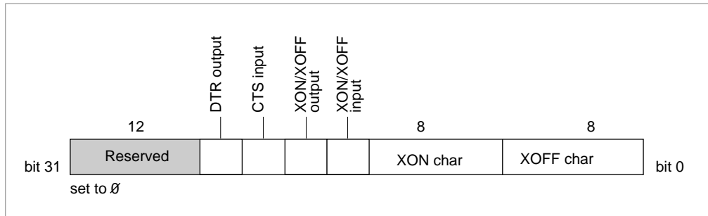
Figure 19-2 Serial port I/O handshaking
