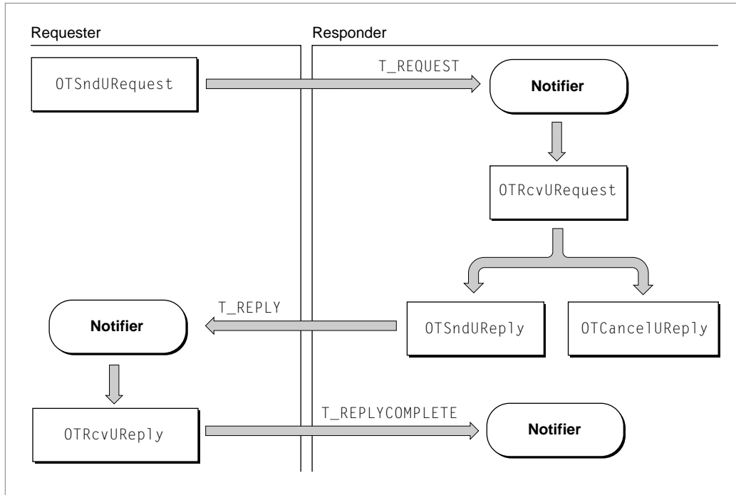
Figure 4-9 Data transfer using connectionless transaction-based endpoints in asynchronous mode
