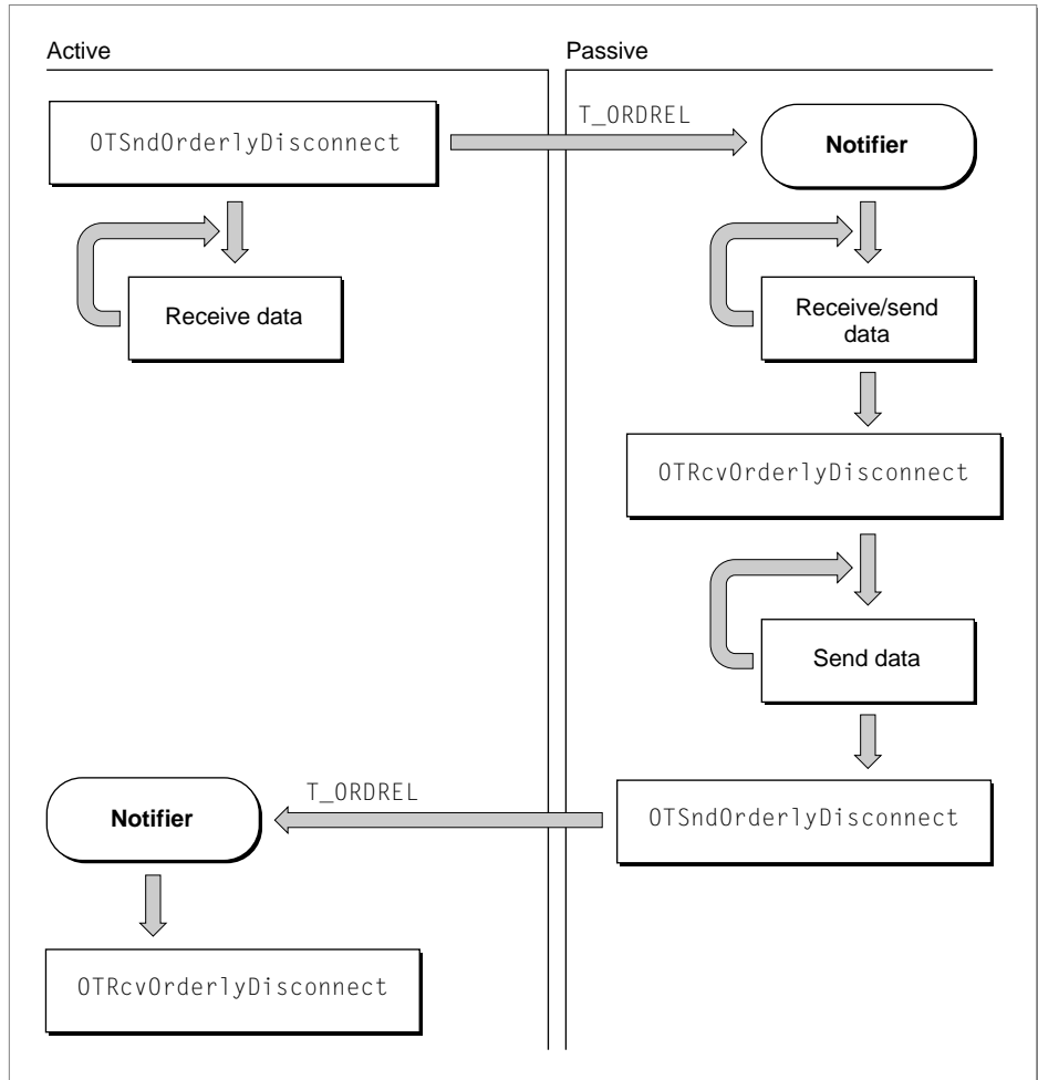
Figure 4-6 Remote orderly disconnect
