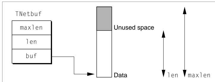
Figure 2-1 The TNetbuf structure
