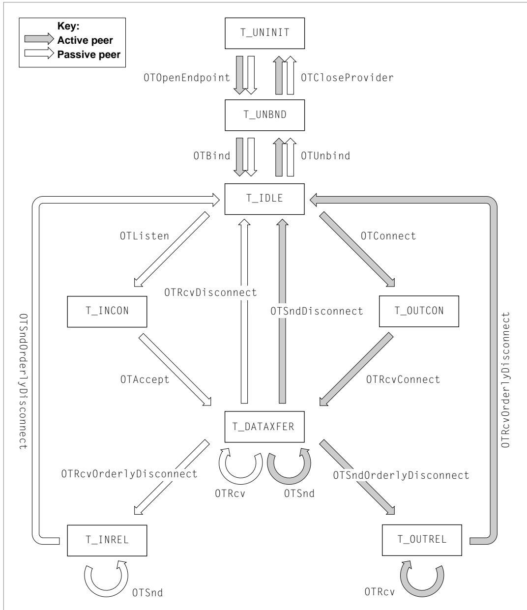
Figure 4-2 Possible endpoint states for a connection-oriented endpoint
