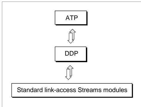
Figure 17-1 The ATP endpoint provider's underlying delivery mechanism
