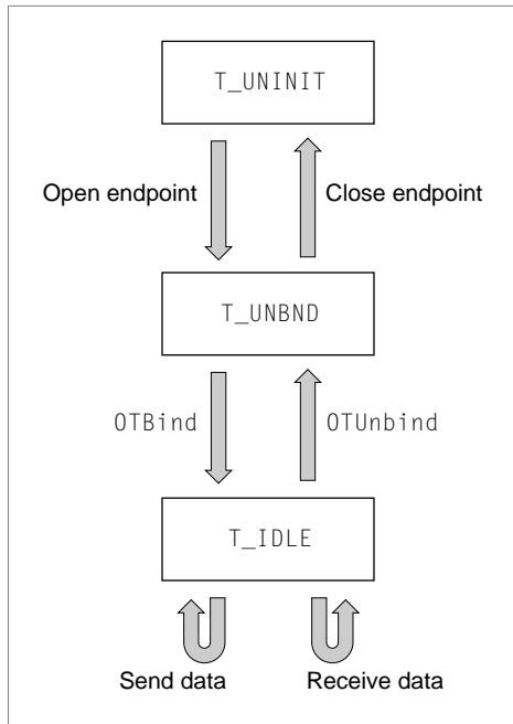
Figure 4-1 Typical endpoint states for a connectionless endpoint
