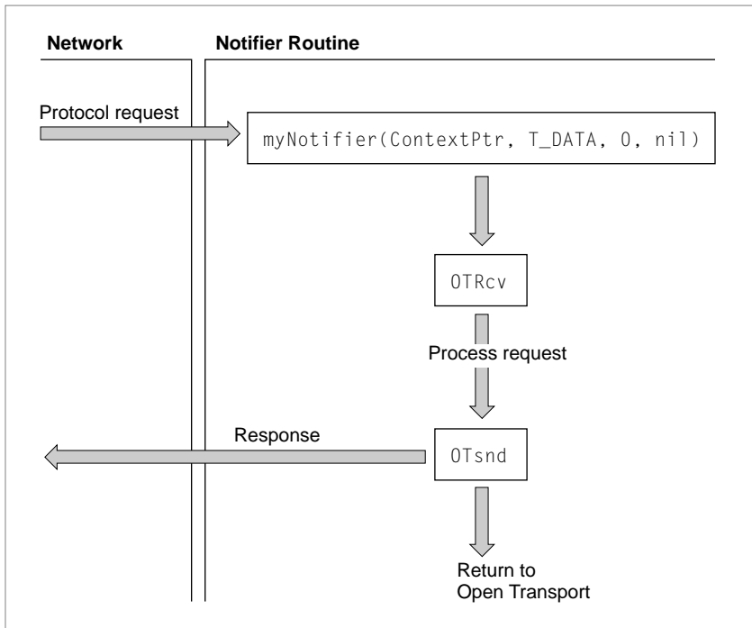
Figure 5-3 Asynchronous processing with a notifier
