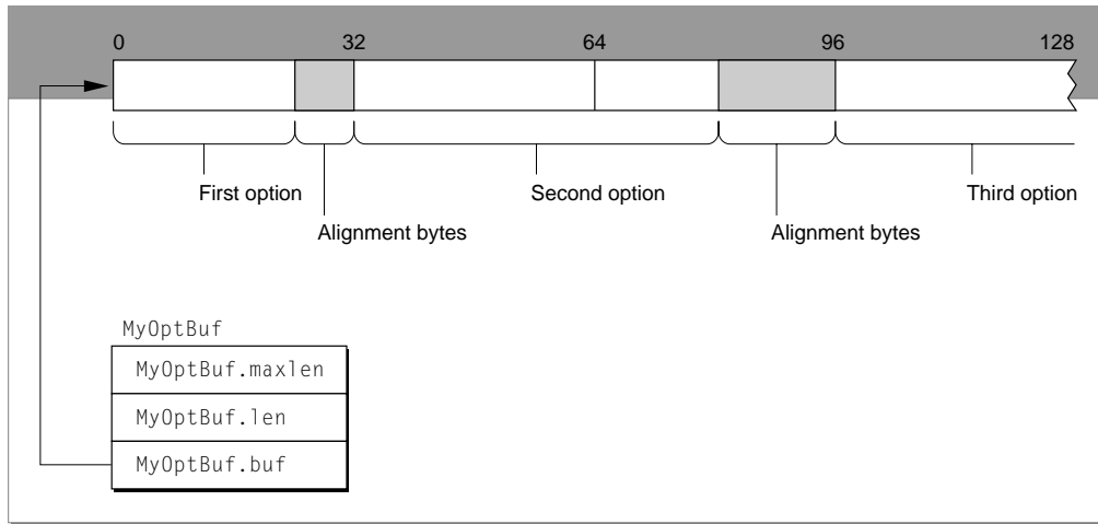
Figure 7-2 An options buffer
