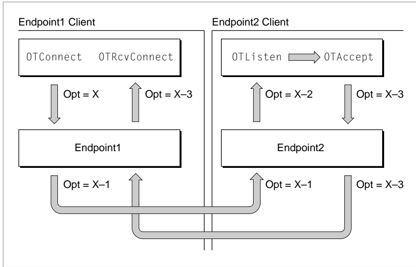
Figure D-1 Negotiating an association-related option
