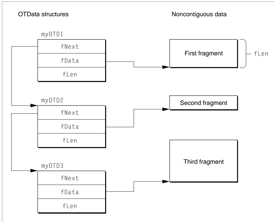
Figure 10-1 Describing noncontiguous data
