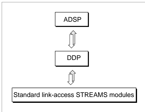
Figure 16-1 The ADSP endpoint provider's underlying delivery mechanism
