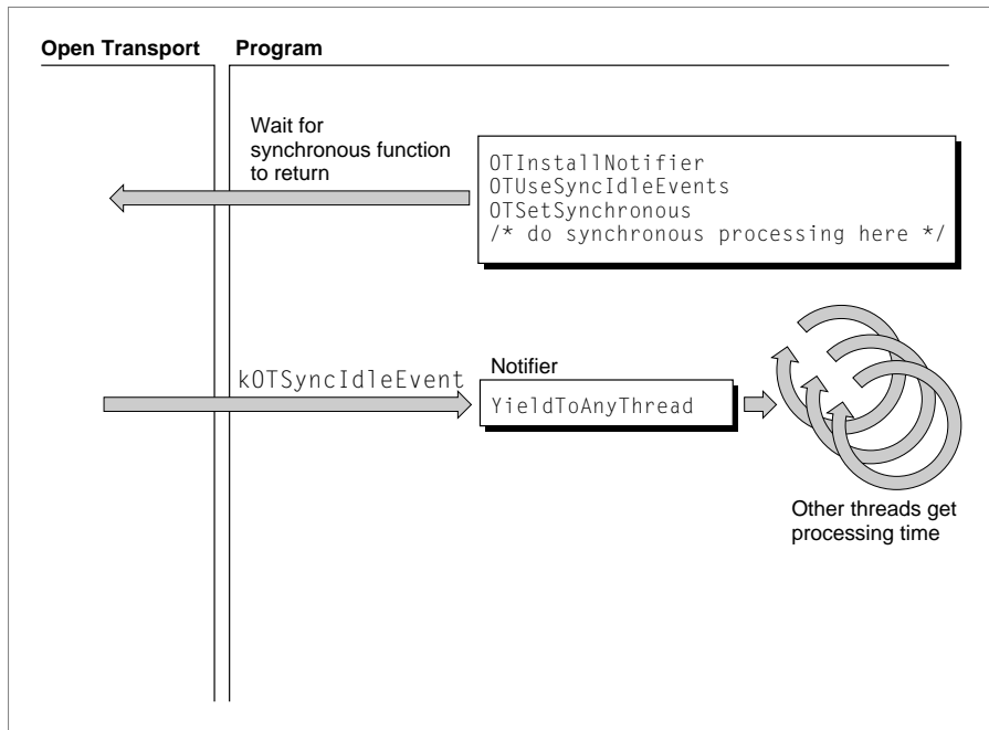
Figure 5-1 Synchronous processing with threads
