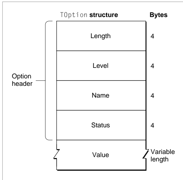
Figure 7-1 The format of option information
