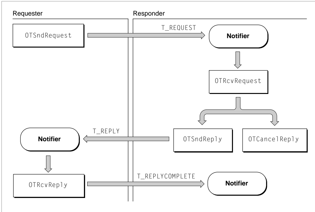
Figure 4-10 Data transfer using connection-oriented transaction-based endpoints in asynchronous mode
