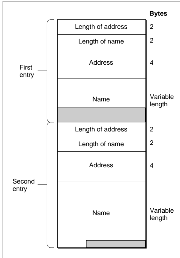
Figure 6-1 Format of entries in OTLookupName reply buffer
