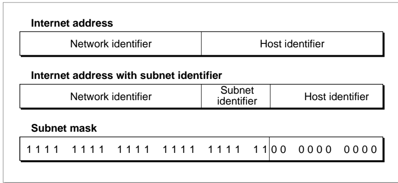
Figure 11-2 Internet subnet address
