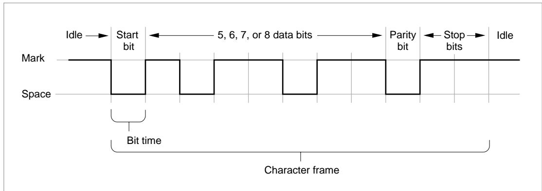
Figure 19-1 The format of serialized bits
