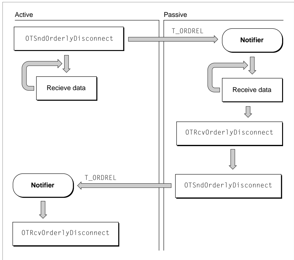
Figure 4-7 A local orderly disconnect
