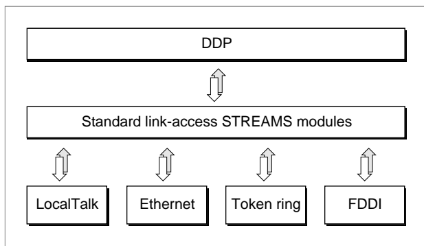
Figure 15-1 The DDP endpoint provider's underlying delivery mechanism
