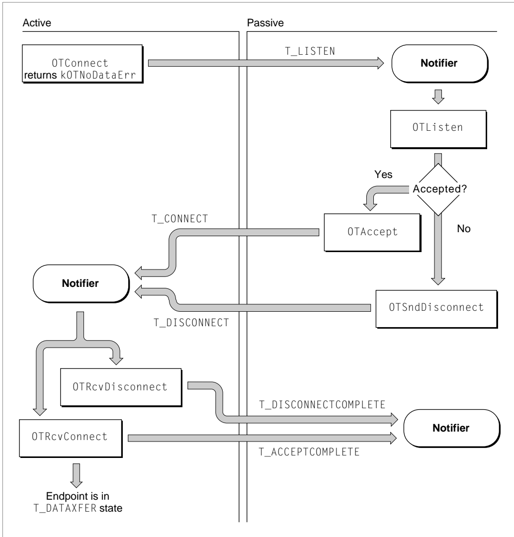
Figure 4-4 Establishing a connection in asynchronous mode
