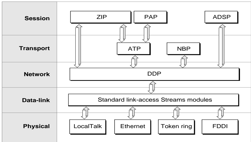
Figure 12-1 AppleTalk protocol stack and the OSI model
