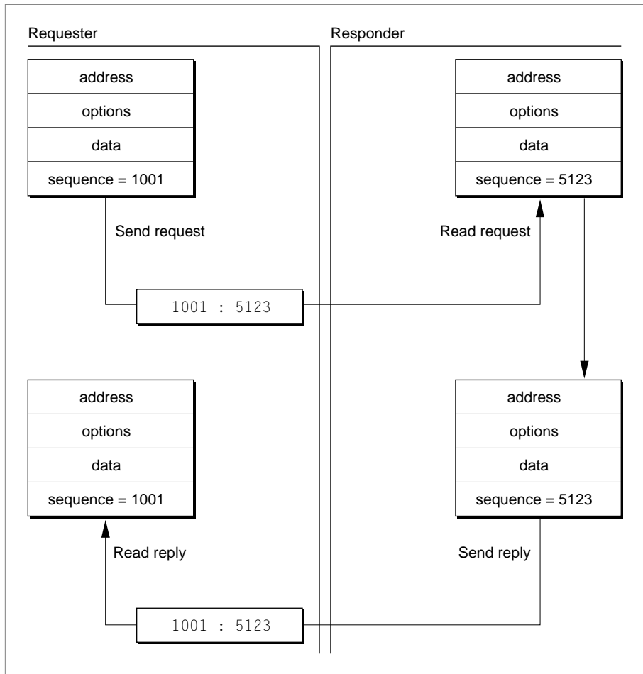
Figure 4-8 How a transaction ID is generated
