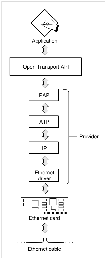
Figure 1-3 An Open Transport Provider
