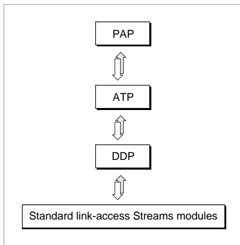
Figure 18-1 The PAP endpoint provider's underlying delivery mechanism
