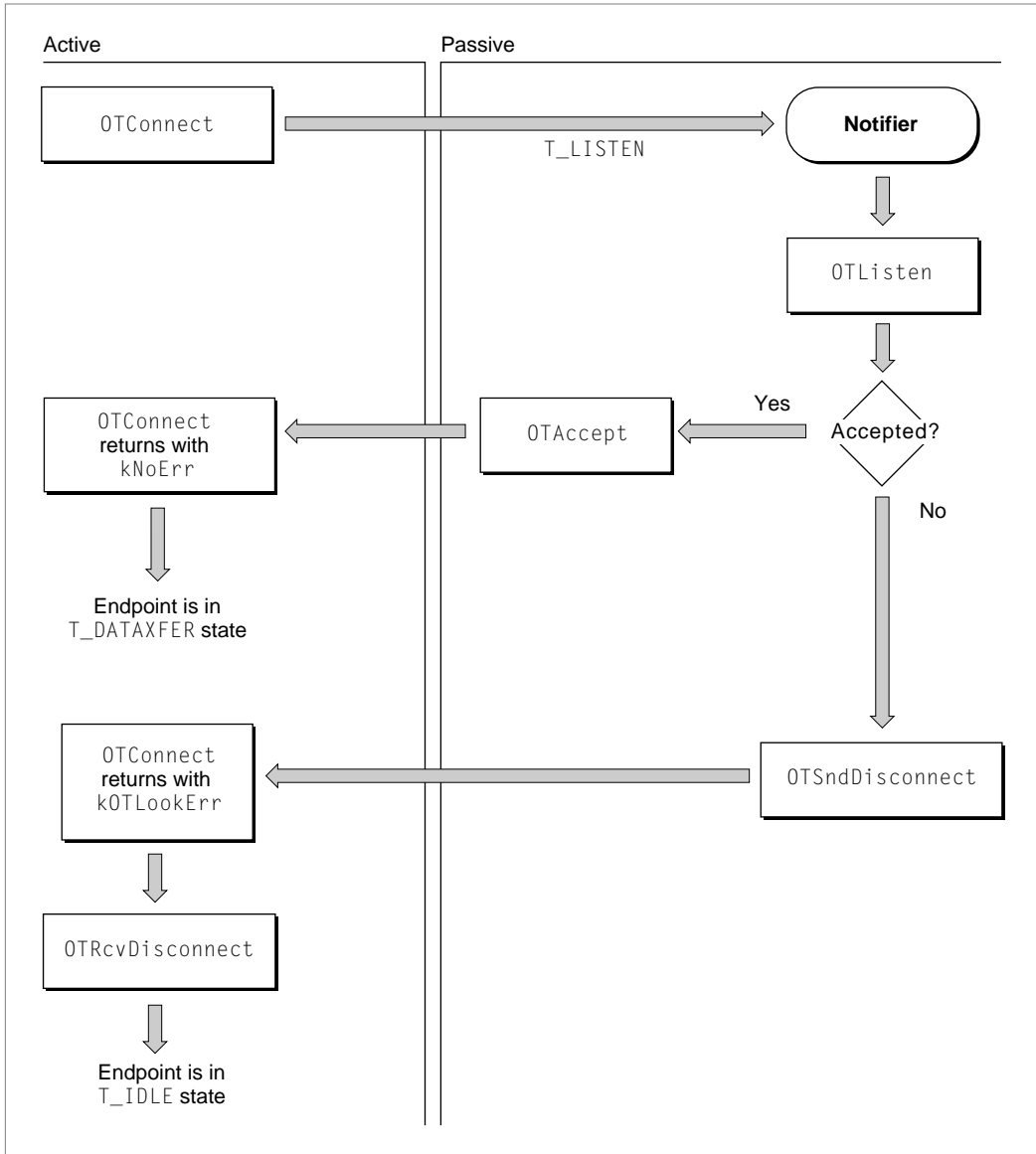
Figure 4-3 Establishing a connection with the active peer in synchronous mode
